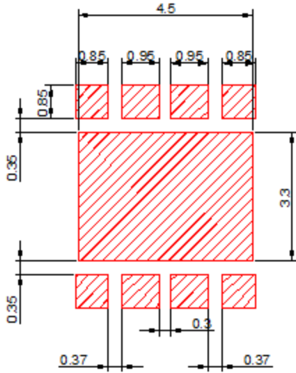
Recommended PCB solder pad
